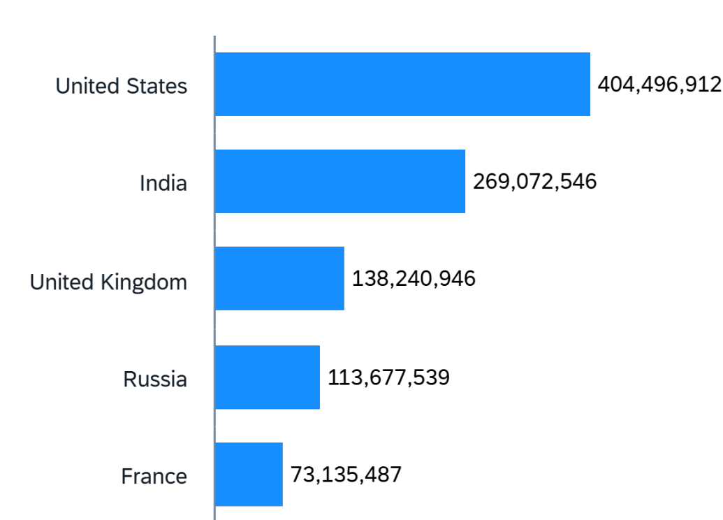
new_tests per location for Actual
